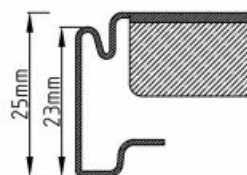
Cefla System 25mm
