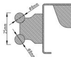
Alser/La Fortezza Double Wire 25mm
