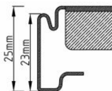
Cefla System 25mm
